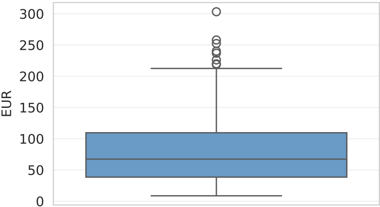
MonthlyRevenue
