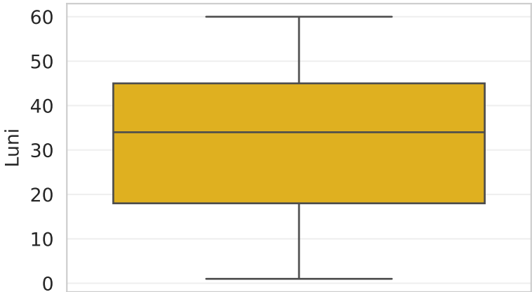
TenureMonths
