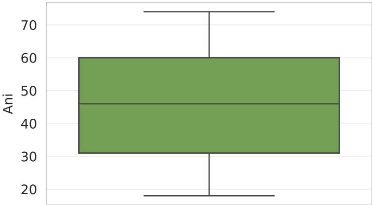
Age
