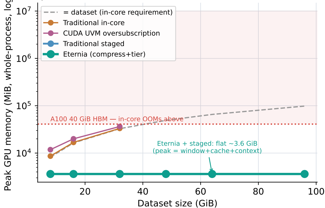
Track A: peak GPU vs size — Eternia bounded/flat, in-core = dataset
