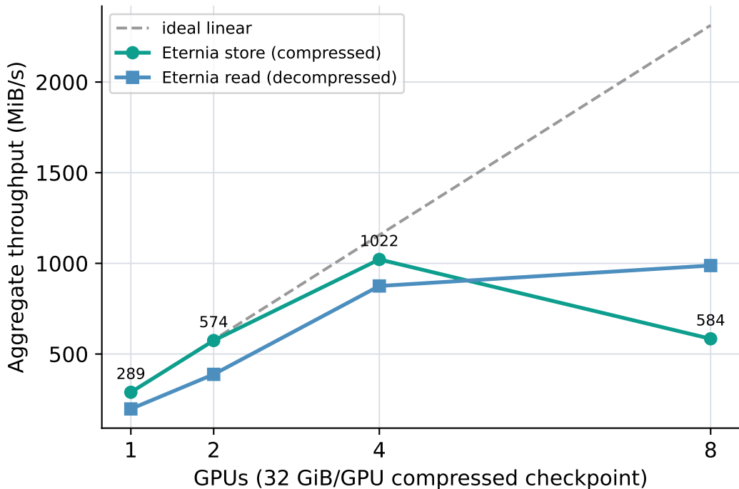
Track B: Eternia distributed weak-scaling (per-GPU cuSZp)
