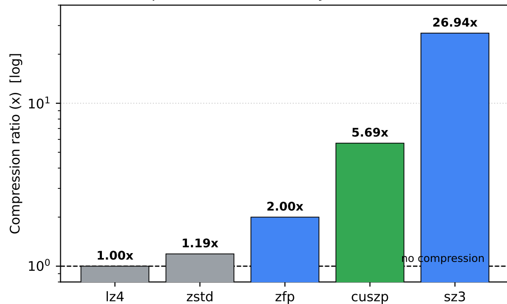
Compression ratio on Gray-Scott float data
