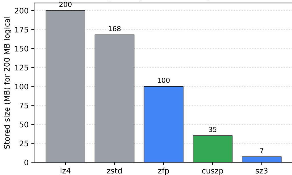
Storage footprint after compression
