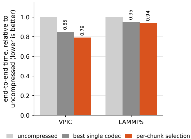
(b) End-to-end time: produce, store, read, analyse
