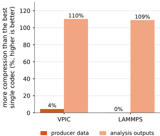
(a) Extra compression from per-chunk selection
