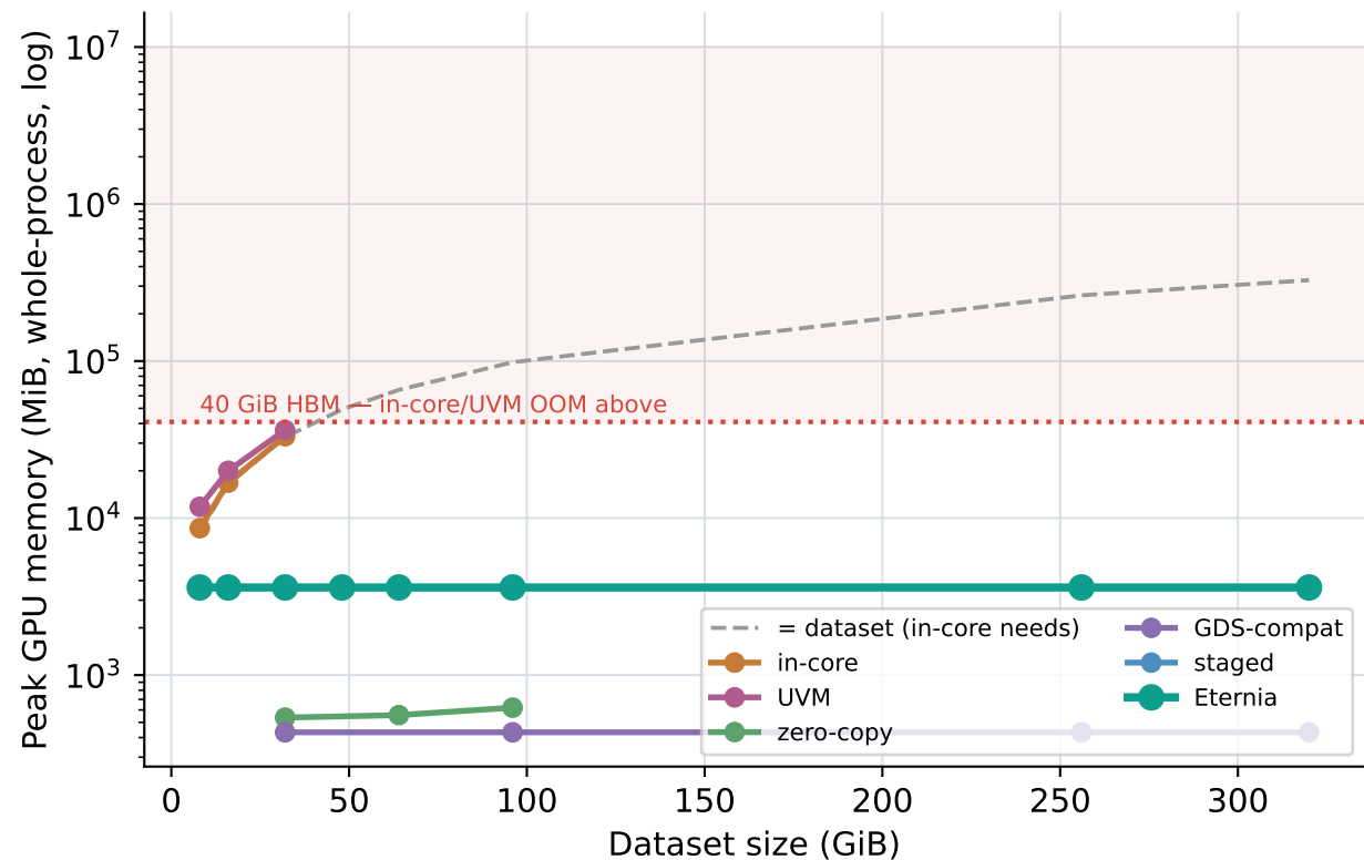
Peak GPU vs size: Eternia bounded/flat ~3.6 GiB; in-core = dataset
