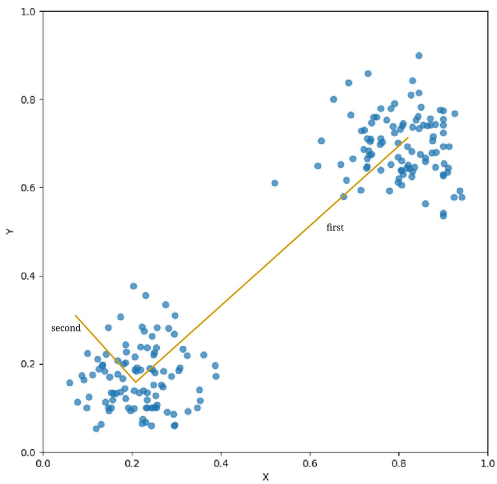
Figure 1: Scatter plot of 2D data points.
