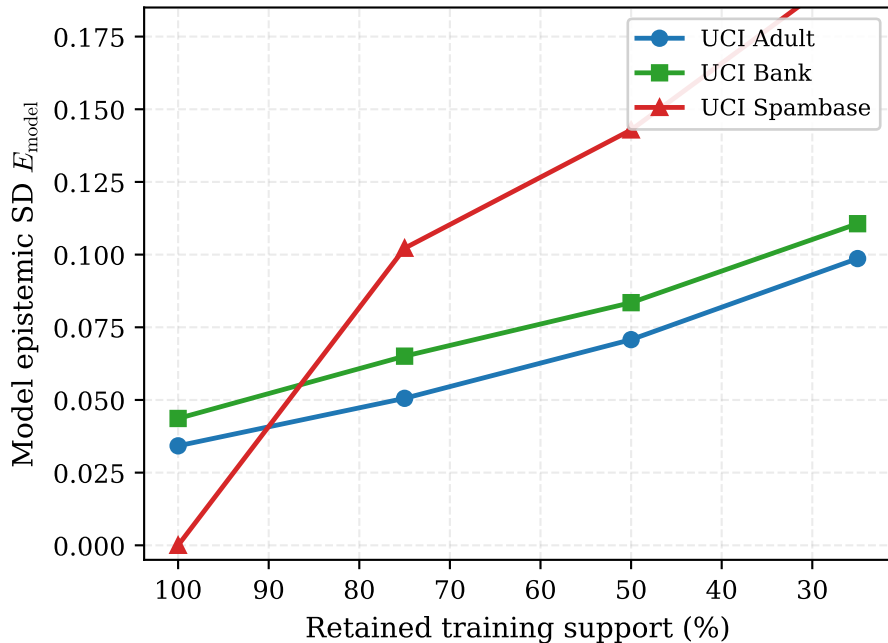
(a) Base model epistemic SD vs. training support
