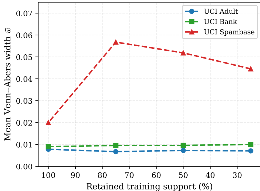
(b) Calibration width under fixed cal support
