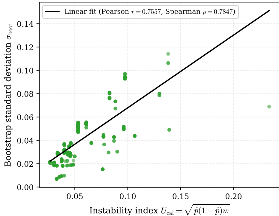
(b) Calibration instability index U_{\text{cal}} vs. \sigma_{\text{boot}}
