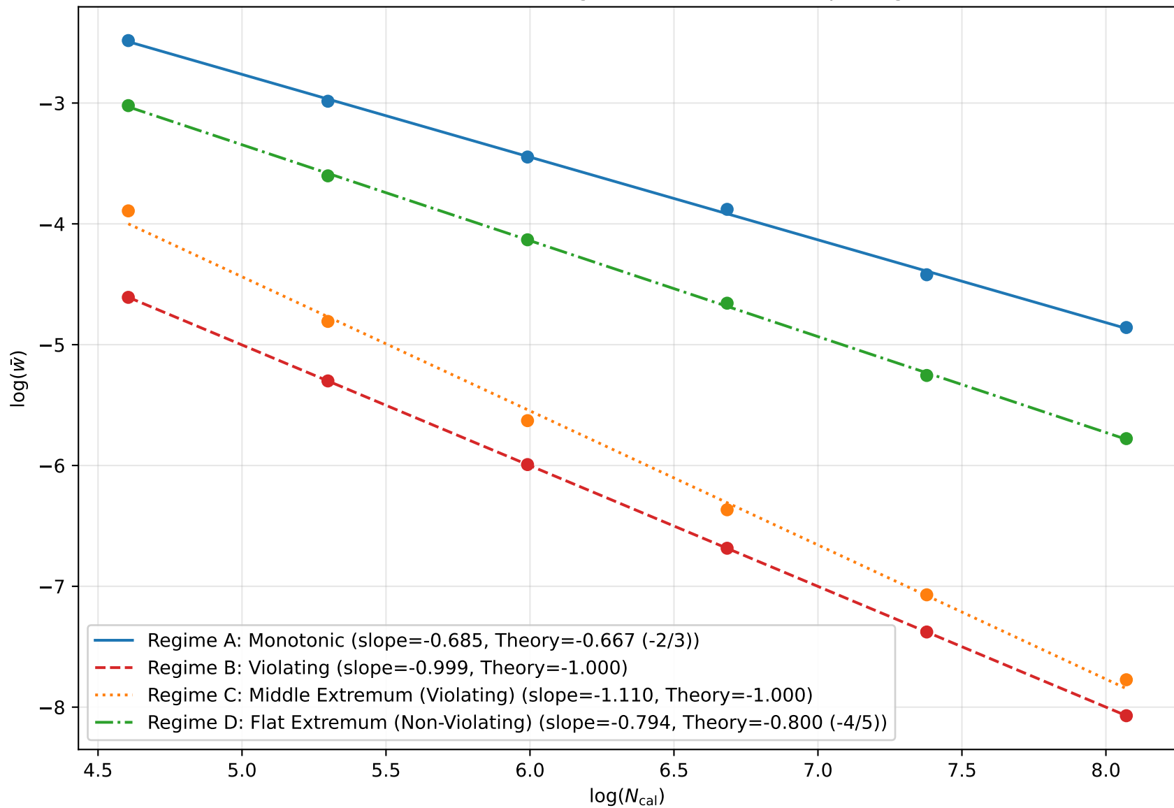
Venn--Abers Width Scaling Laws in Different Slope Regimes
