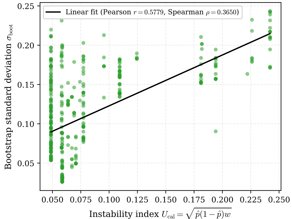
(b) Calibration instability index U_{\text{cal}} vs. \sigma_{\text{boot}}
