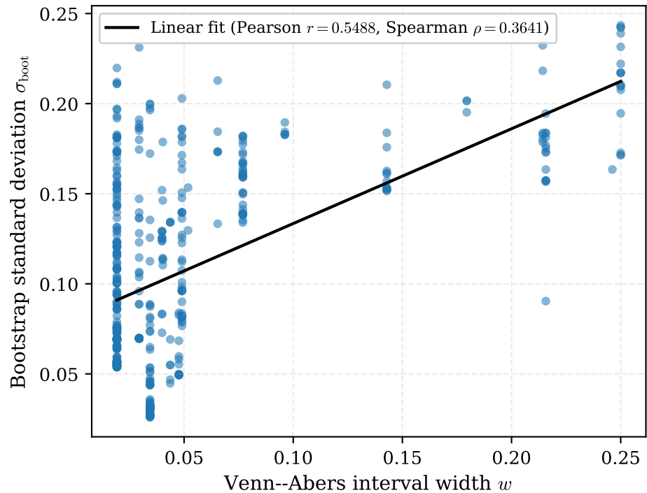
(a) Raw interval width w vs. \sigma_{\text{boot}}
