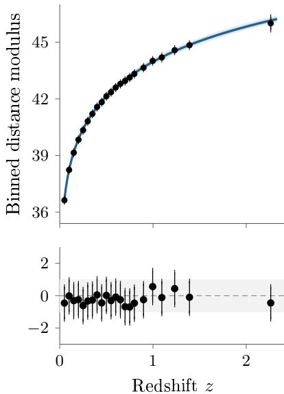
(b) Union3 supernovae
