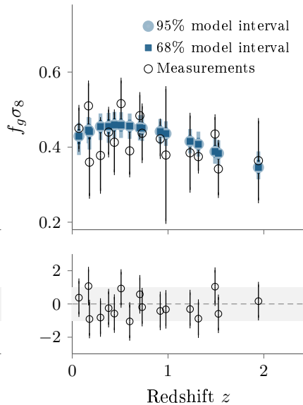
(c) Growth compilation
