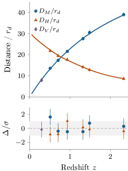
(a) DESI DR2 BAO
