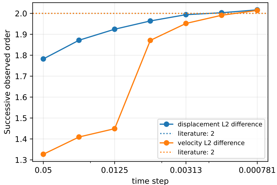
Elastodynamic MHM — time refinement
