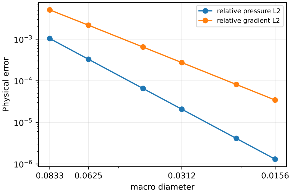
Helmholtz MHM
