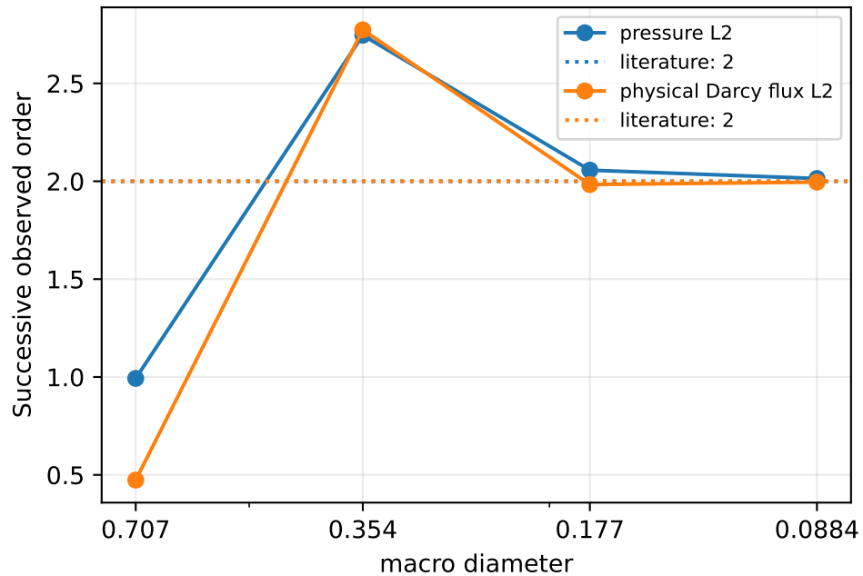
MHM with mixed H(div) locals
