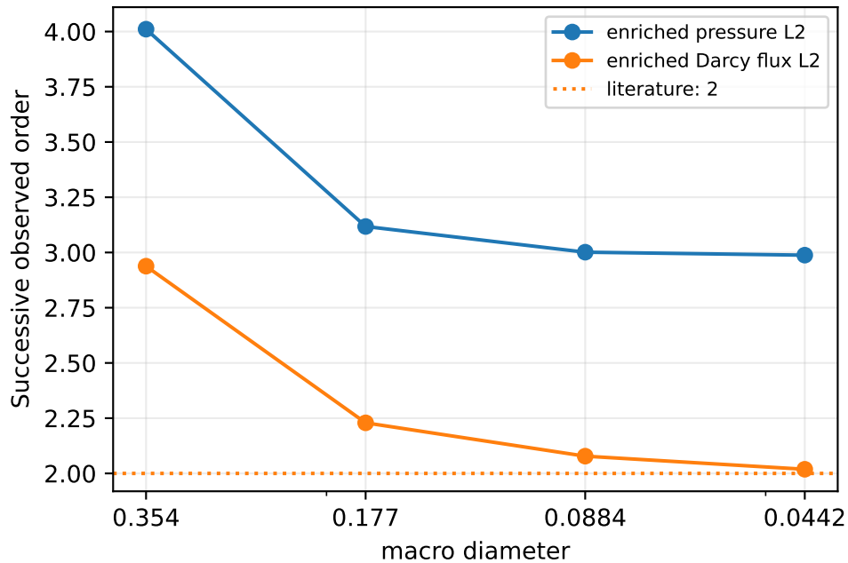
Petrov-Galerkin MHM
