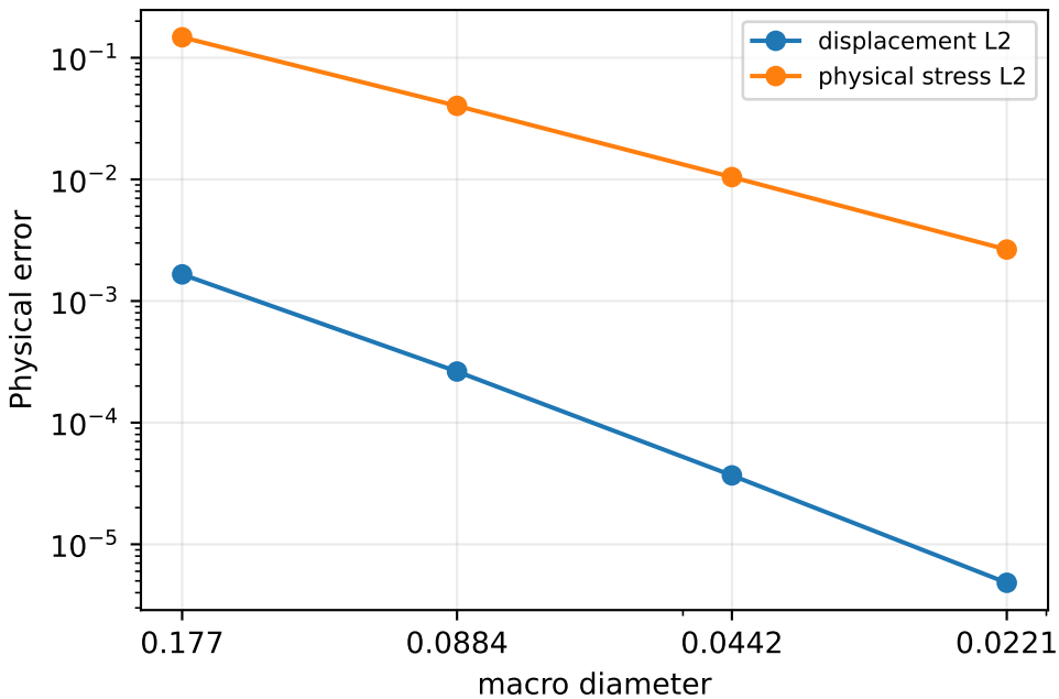
Primal elasticity MHM
