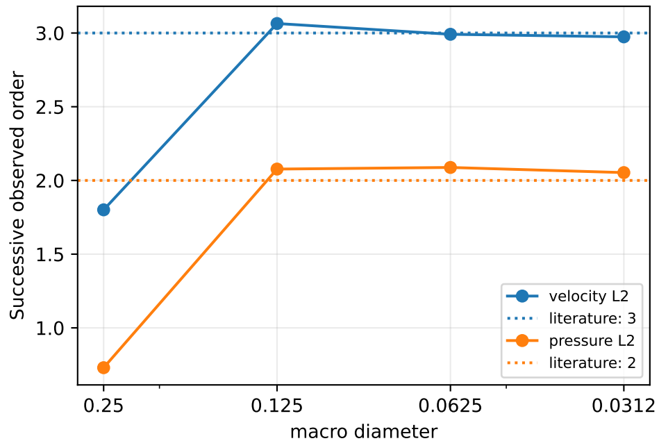
Stokes-Brinkman MHM
