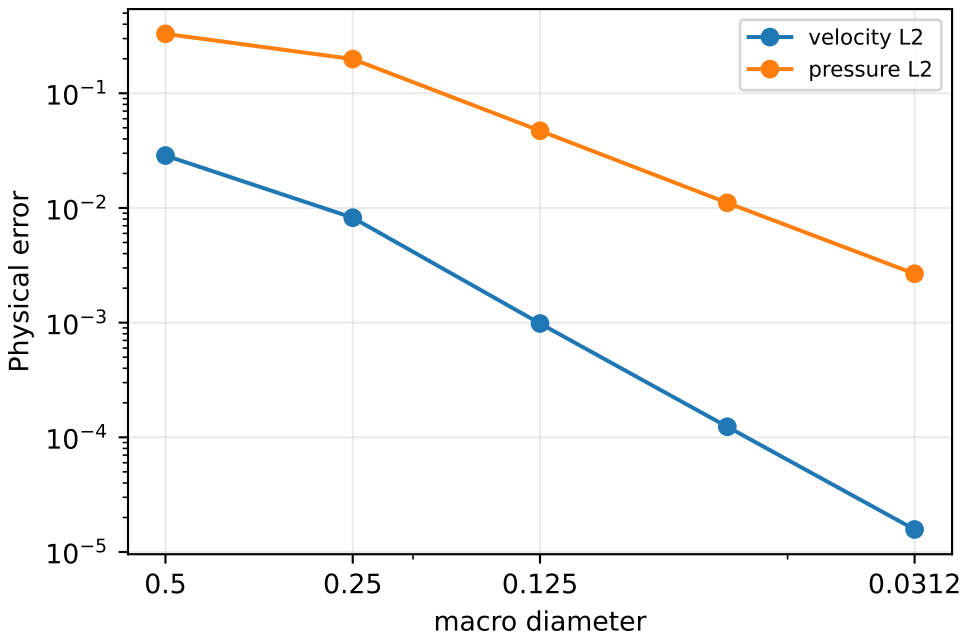
Stokes-Brinkman MHM
