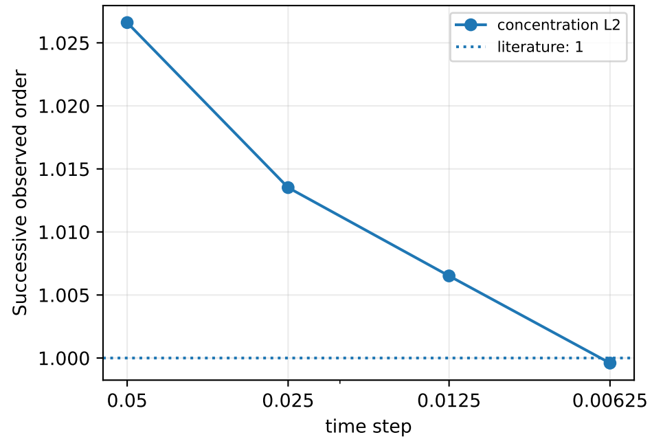
Transient transport MHM — time refinement
