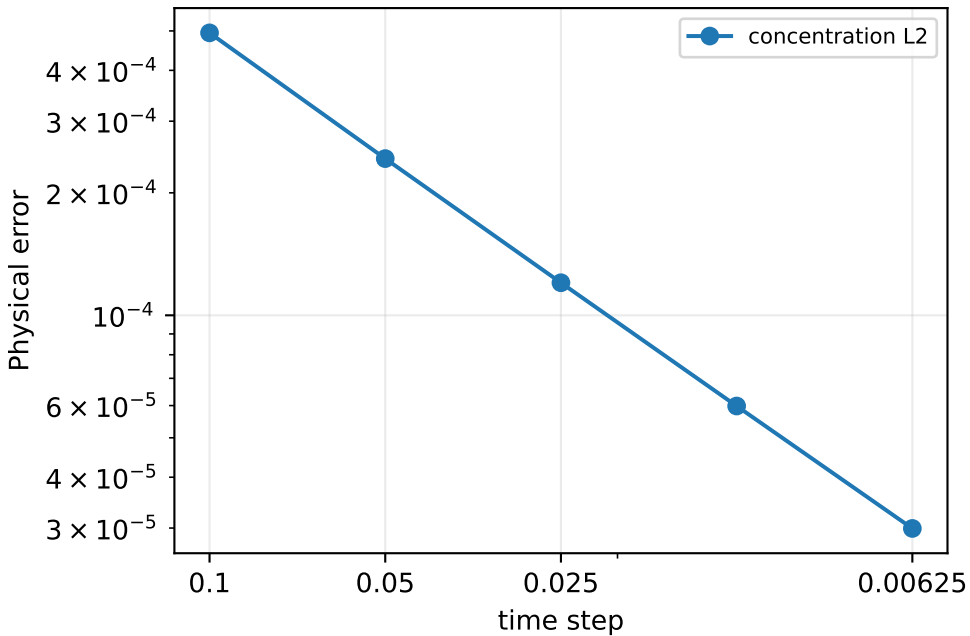
Transient transport MHM — time refinement
