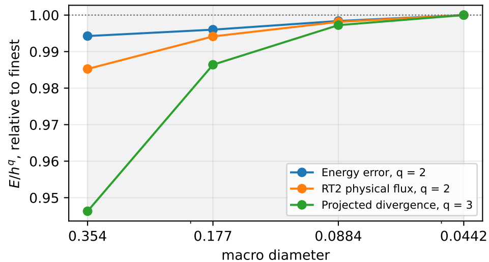
Target-normalized errors
