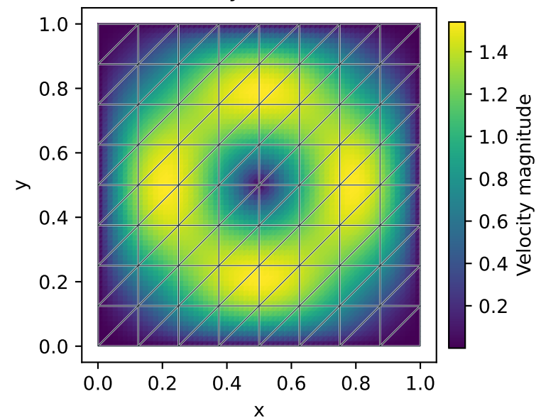
Classical Taylor-Hood: n=64
