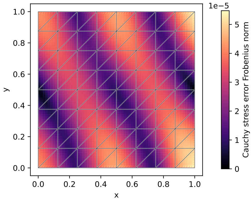
Classical P3: n=64
