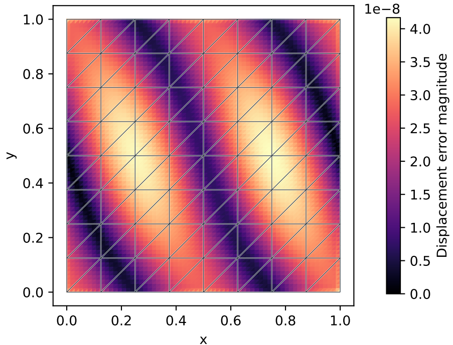
Classical P3: n=64
