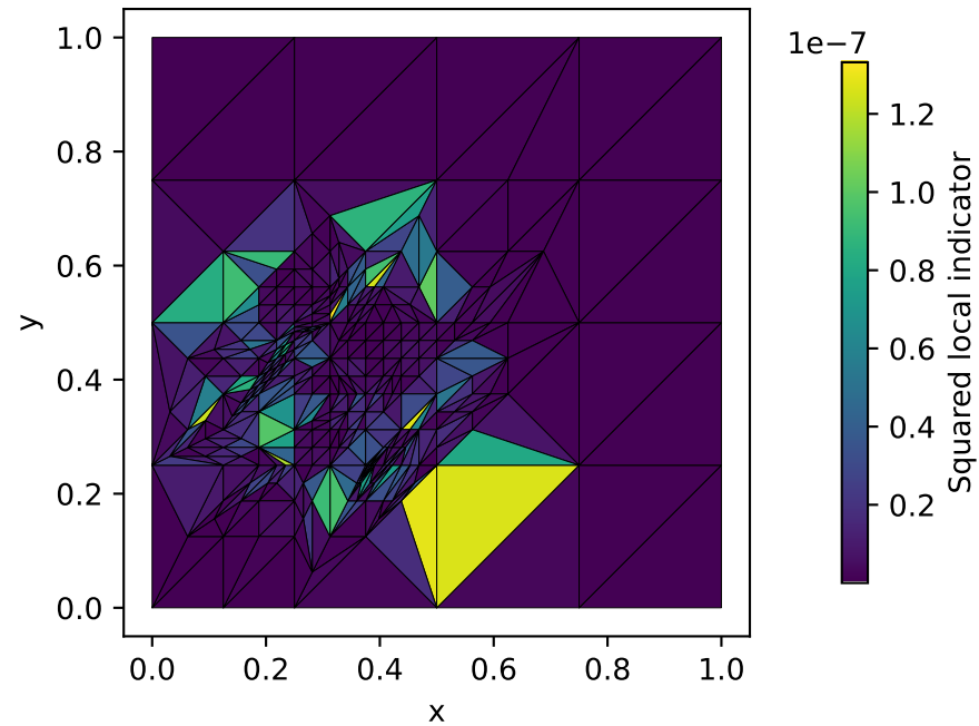
Final adaptive macro mesh 507 cells
