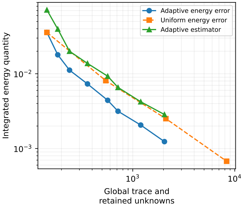
Localized smooth solution Error and work
