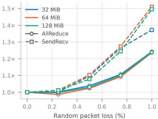
(b) Packet loss
