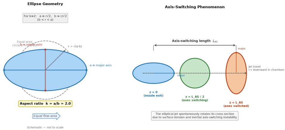
Figure 3: Elliptical nozzle geometry (left) and axis-switching sequence (right). The dashed circle shows the equal-area circular orifice; the ellipse minor axis b is smaller by a factor 1/\sqrt{k} , producing finer minimum droplets.
