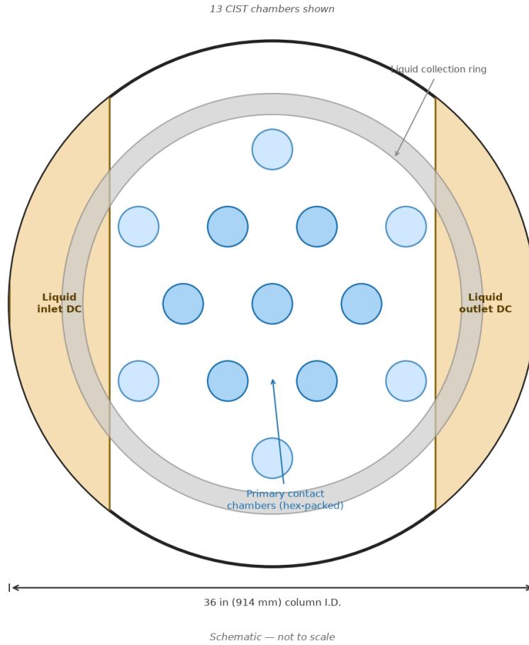
Fig. 2 — CIST Tray Plan View
