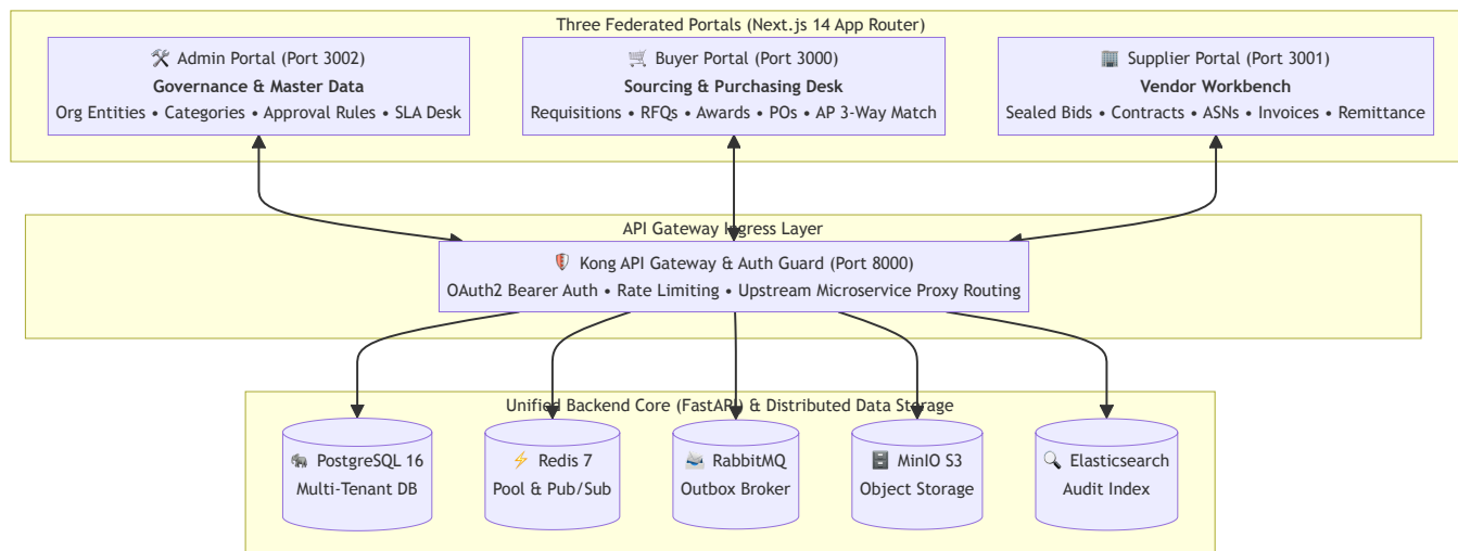
Figure 1.1: Platform Topology & Multi-Portal Interconnect over Kong API Gateway
