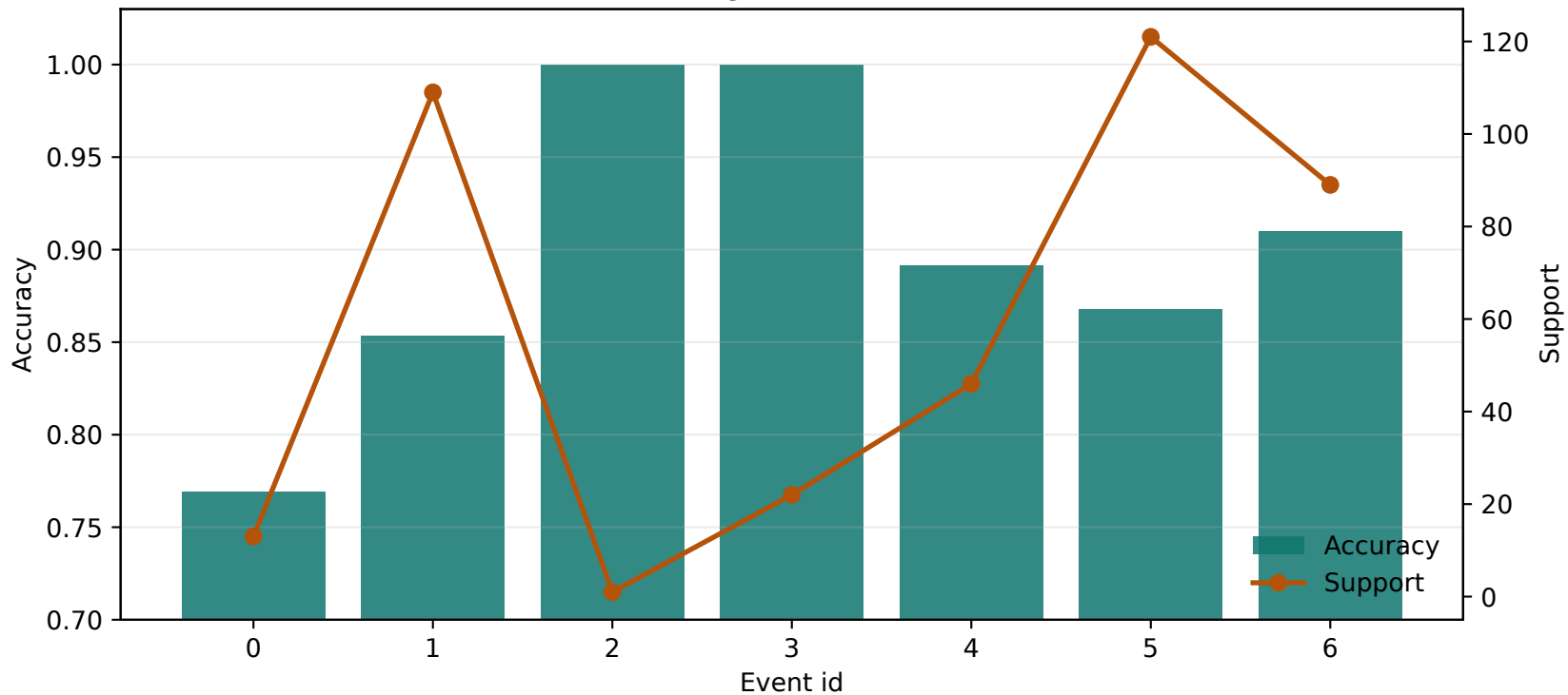
Event-level generalization check
