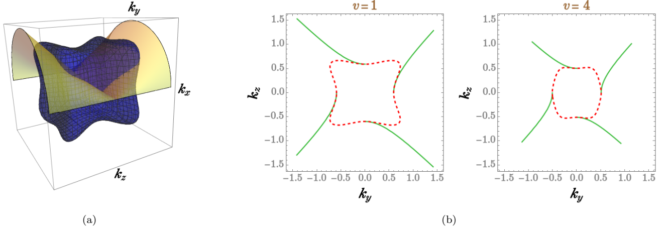
FIG. 6. (a) The FS-projection is obtained by cutting the 3d FS with the yellow-coloured 2d surface, captured by Eq. (44). Here, \mu = 0.25 and v = 1 . (b) The Fermi arcs represent modes with E = \mu , where \mu = 0.25 . The dashed red closed contour represents the projection of the bulk FS on the k_y k_z -plane.
