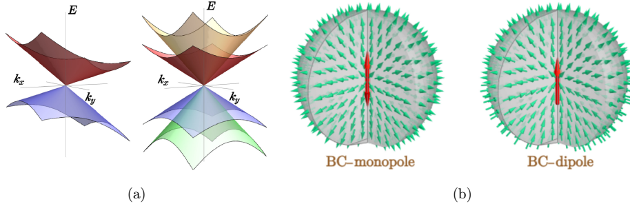
Fig. 1. (Color online) (a) Dispersion ( E ) of the bands, crossing at a tilted Weyl node and a fourfold-degenerate RSW node, against the k_x k_y -plane. (b) Schematics of BC-flux field in the 3d momentum space for a monopole and an ideal dipole.
