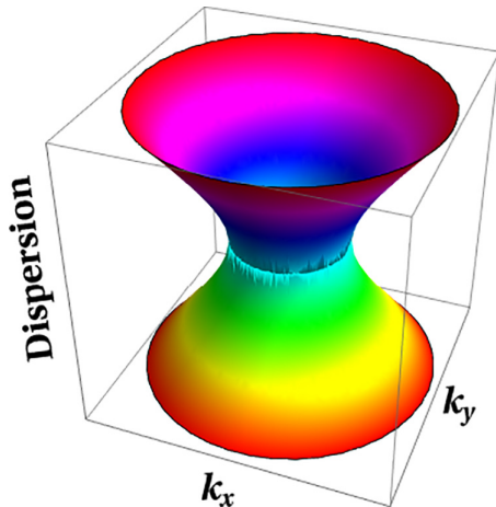
FIG. 2. A third-order exceptional circle (EC 3 ) for a three-band model, exemplified by Eq. (19), showing square-root singularities.
