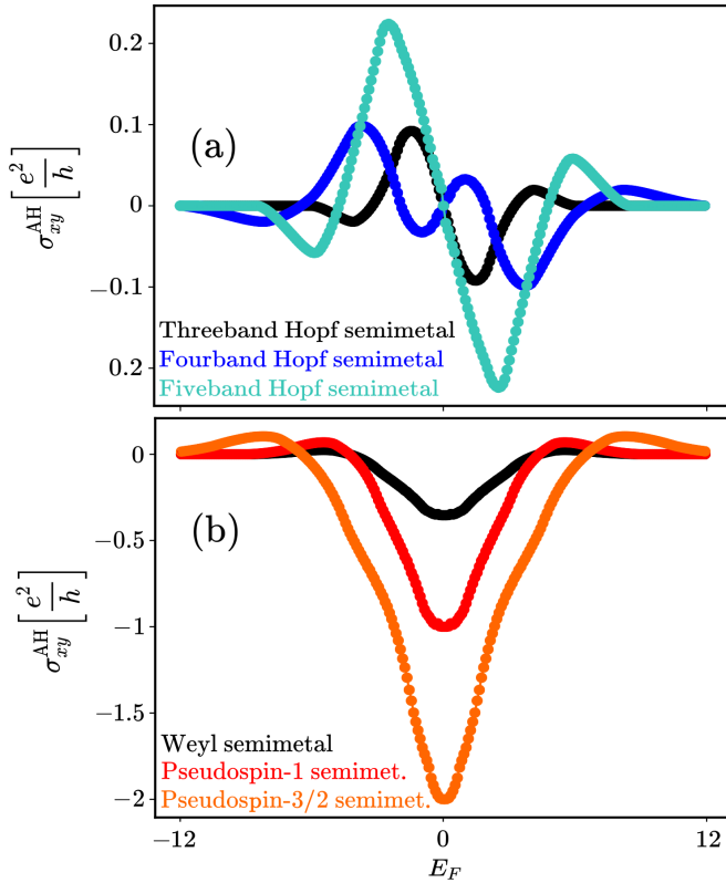
FIG. 3. (a) Anomalous Hall conductivity for lattice models \hbar_N(\mathbf{k}) [cf. Eq. (19)] of massless multifold Hopf semimetals. The parameter \Delta_0 = -3 is chosen such as to ensure the existence of a single Berry dipole at the \Gamma point, described by a continuum Hamiltonian (4). The odd parity of the AH conductivity is due to the property \kappa_\alpha = \kappa_{-\alpha} of the geometric charges of this Berry dipole. (b) Typical anomalous Hall conductivity for lattice models of chiral topological semimetals with a single pair of Berry monopoles [cf. Eq. (F4)]. The even parity is due to the property C_\alpha = -C_{-\alpha} of the Chern number associated to each Berry monopole.
