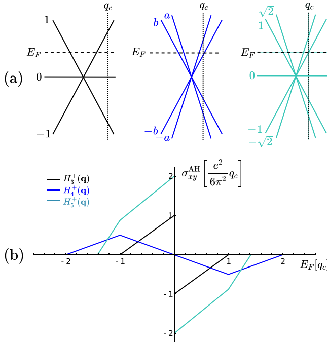
FIG. 10. (a) Schematic energy spectrum of the Hopf semimetal continuum models H_{N=3,4,5}^{\xi=\pm}(\mathbf{q}) with Fermi energy E_F , momentum cutoff q_c , and band velocities c_a indicated. (b) Corresponding anomalous Hall conductivity. For N = 4 , we have used band velocities a = 2, b = 1 . For N odd, there is an abrupt sign change at half filling, with a jump equal to the Berry dipole charge \kappa_0 of the flat band.
