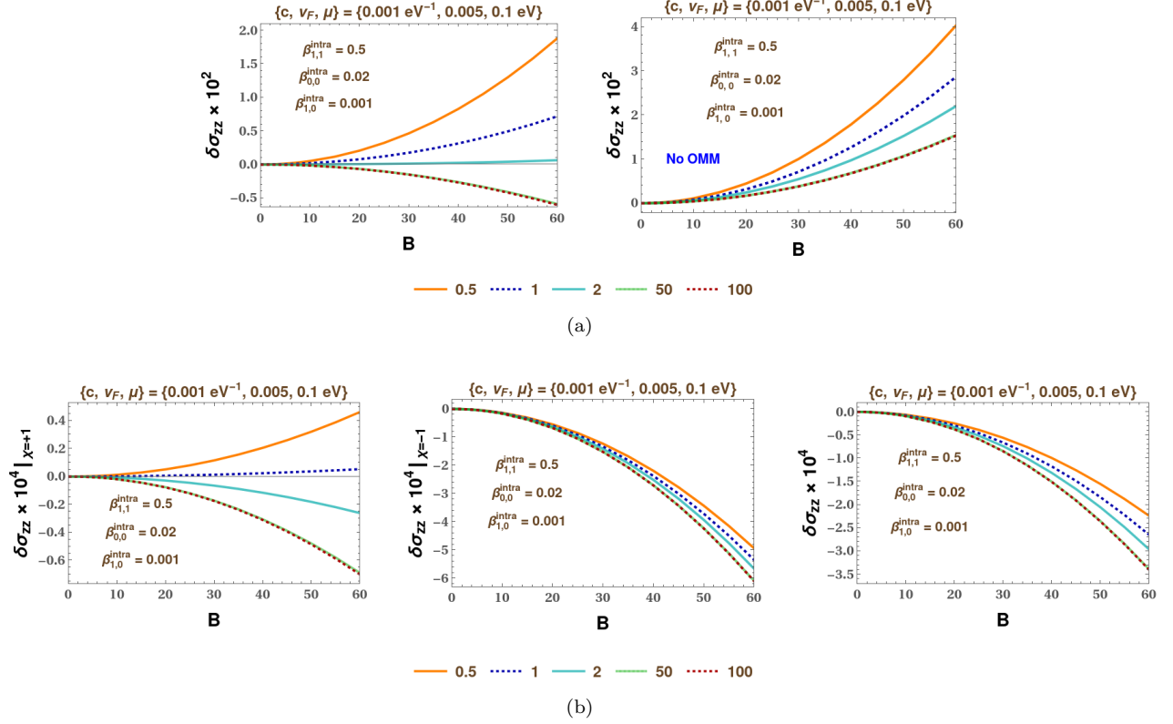
FIG. 6. (a) Net \delta\sigma_{zz} from the \{s, \tilde{s}\} = \{1, 1\} bands, when interacting mutually and with the \{s, \tilde{s}\} = \{0, 0\} bands, as B (in \text{eV}^2 ) is cranked up. (b) Node-dependent and net values of \delta\sigma_{zz} for the \{s, \tilde{s}\} = \{0, 0\} bands, as B is varied, when interacting mutually and with the \{s, \tilde{s}\} = \{1, 1\} bands. The plot-legends indicate the values of the ratios \{\beta_{s,\tilde{s}}^{\text{inter}}/\beta_{s,\tilde{s}}^{\text{intra}}\} .
