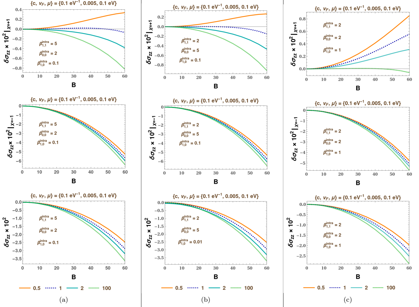
FIG. 5. \delta\sigma_{zz} from the \{s, \tilde{s}\} = \{0, 0\} bands interacting mutually and with the \{s, \tilde{s}\} = \{1, 1\} bands: The curves demonstrate the variation of conductivity with B (in \text{eV}^2 ). The top, middle, and bottom panels represent the results for the \chi = +1 node, \chi = -1 node, and sum over both the nodes, respectively. The plot-legends indicate the values of the ratios \{\beta_{s,\tilde{s}}^{\text{inter}}/\beta_{s,\tilde{s}}^{\text{intra}}\} . The three subfigures represent three distinct sets of parameter values, as indicated in the labels.
