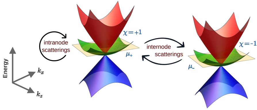
FIG. 1. Schematics of the scattering processes between two nodes in a TSM, carrying opposite values of chirality. The values of the chemical potential, represented by the yellow planes, have been tuned to cut the positive-energy bands at each node.
