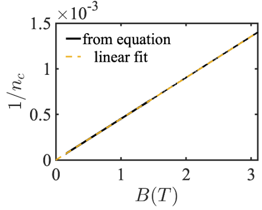
Figure 10. 1/n_c as a function of the magnetic field, where n_c is the number of occupied Landau levels. Figure adapted from Ref. [67].
