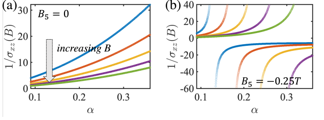
Figure 19. Planar Hall conductance for a minimal model of untitled WSM as a function of intervalley scattering strength. (a) in absence of B_5 field. (b) in presence of B_5 field. In all the curves, as we go from blue to green, we increase B . All the plots are appropriately normalized. Figure adapted from Ref. [69].
