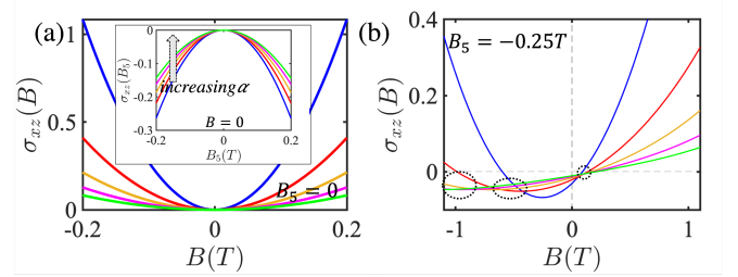
Figure 18. Planar Hall conductivity for a minimal model of untitled TR broken WSM. (a) PHC as a function of the external magnetic field B and no strain-induced field ( B_5 = 0 ). Inset: PHC has been plotted as a function of B_5 with no external field ( B = 0 ). The angle \gamma was chosen to be equal to \gamma_5 . (b) PHC in the presence of both magnetic field and strain. The chiral gauge field causes weak sign-reversal. The dotted ellipses highlight regions that show an anomalous behavior with respect to intervalley scattering strength. All the plots are appropriately normalized. Figure adapted from Ref. [69].
