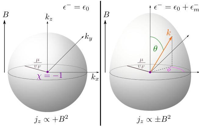
FIG. 1. Sketch of the Fermi surface surrounding a Weyl node if the OMM is not (left) or is (right) taken into account. The inclusion of the OMM leads to an egg-shaped Fermi surface, and the magnetoconductance can be either positive or negative, depending on the scattering amplitudes.
