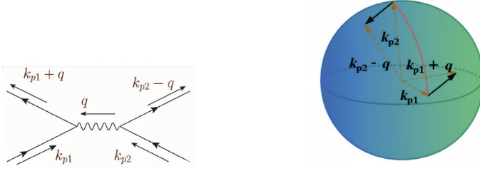
Fig. 2.2 For a FS with dimension m > 1 , any two points on the FS have a common tangent space which is (m - 1) -dimensional
