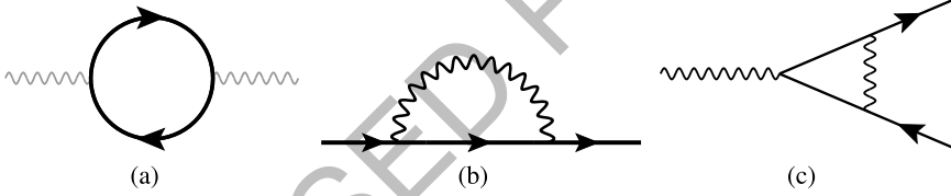
Fig. 2.4 The one-loop diagrams for the a bosonic self-energy, b fermionic self-energy, and c vertex correction. In (a) , the gray wiggly curve denotes the bare bosonic propagator. The solid arrows represent bare fermionic propagators, while the wiggly curves in (b) and (c) denote dressed bosonic propagators that incorporate the one-loop self-energy shown in (a)
