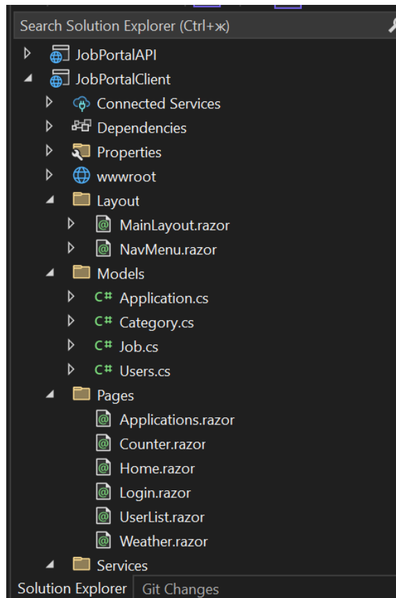
Fig 1 – Structure of the project
