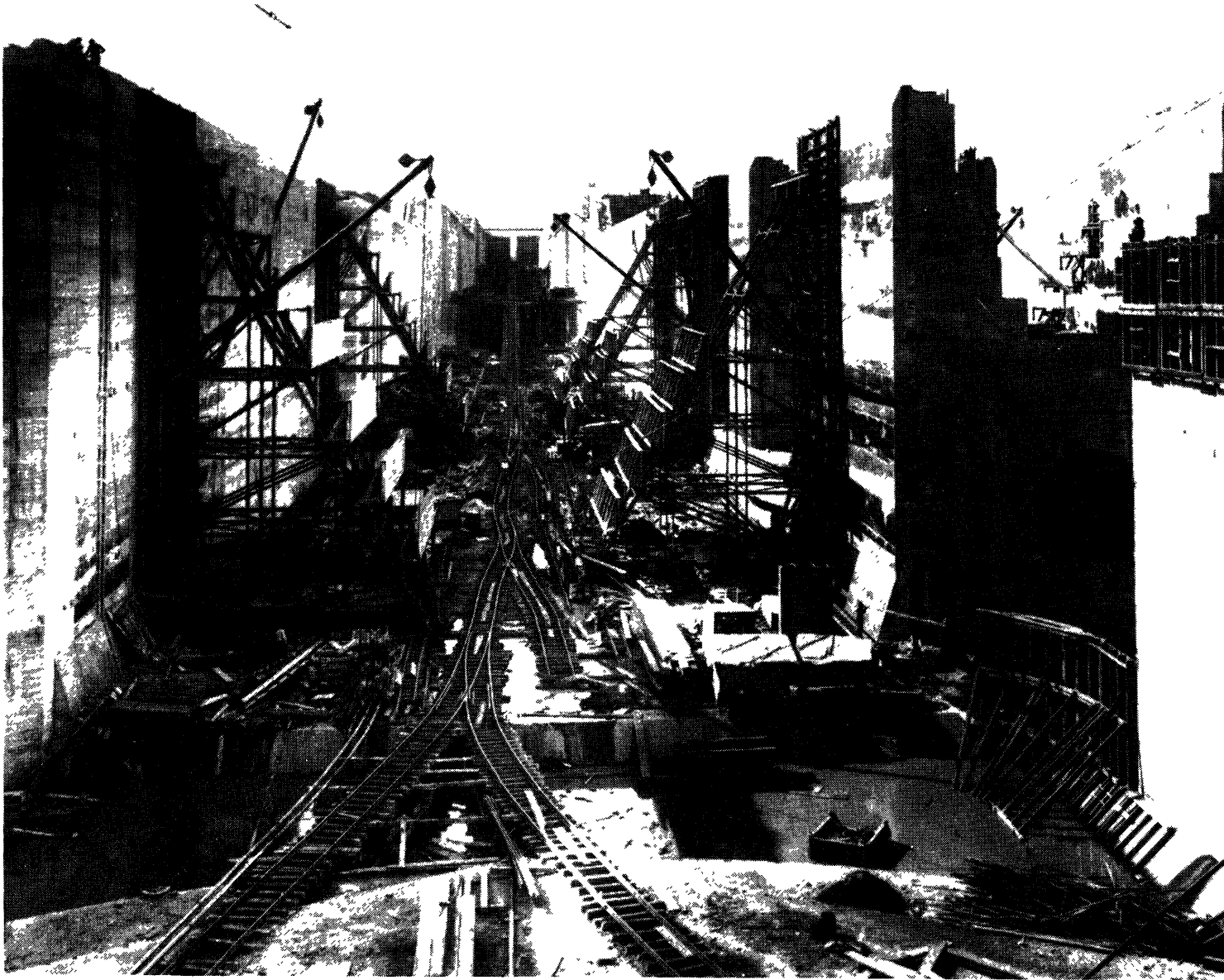
The east chamber of Gatun Lower Locks during construction. The middle and upper locks are in the distance.
