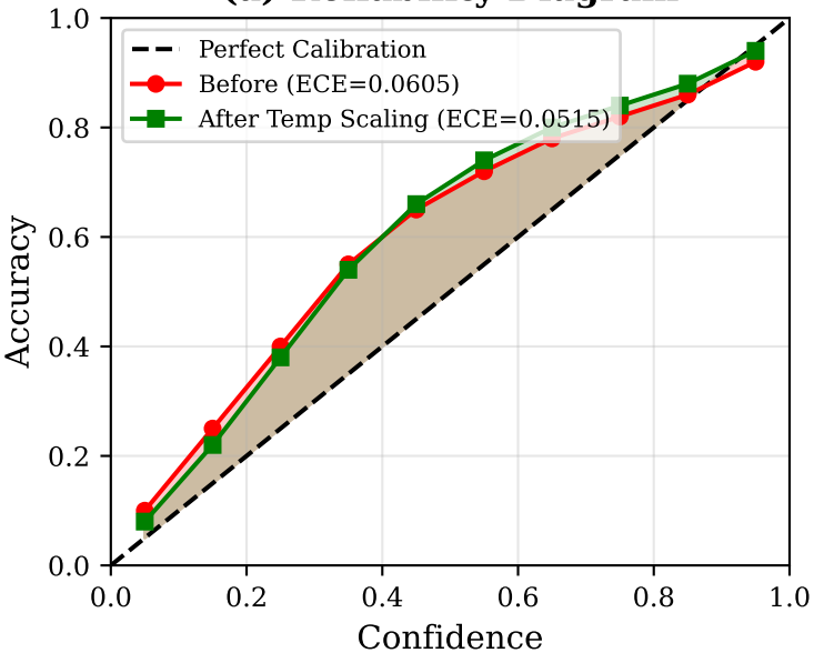
(a) Reliability Diagram
