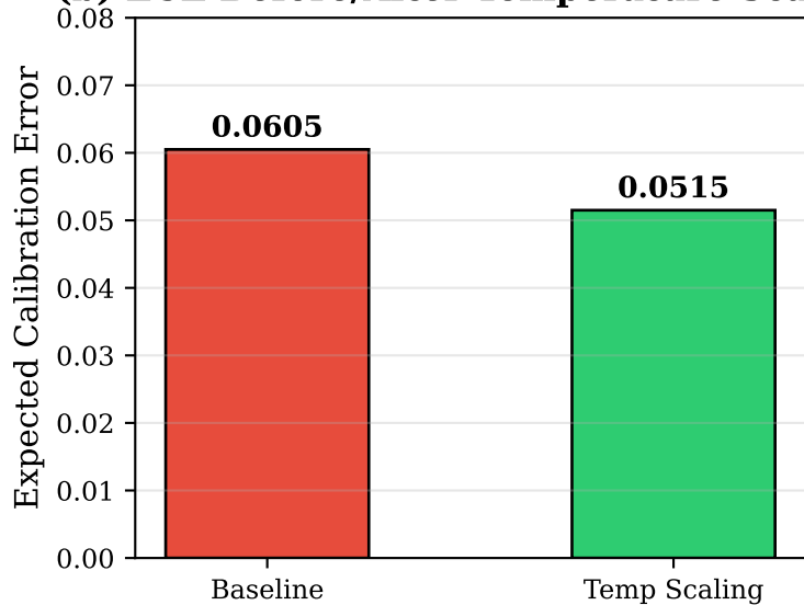
(b) ECE Before/After Temperature Scaling
