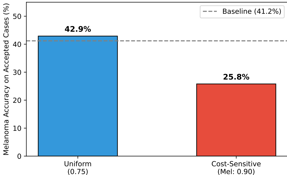
(g) Cost-Sensitive Rejection: Higher Threshold = Worse Accuracy
