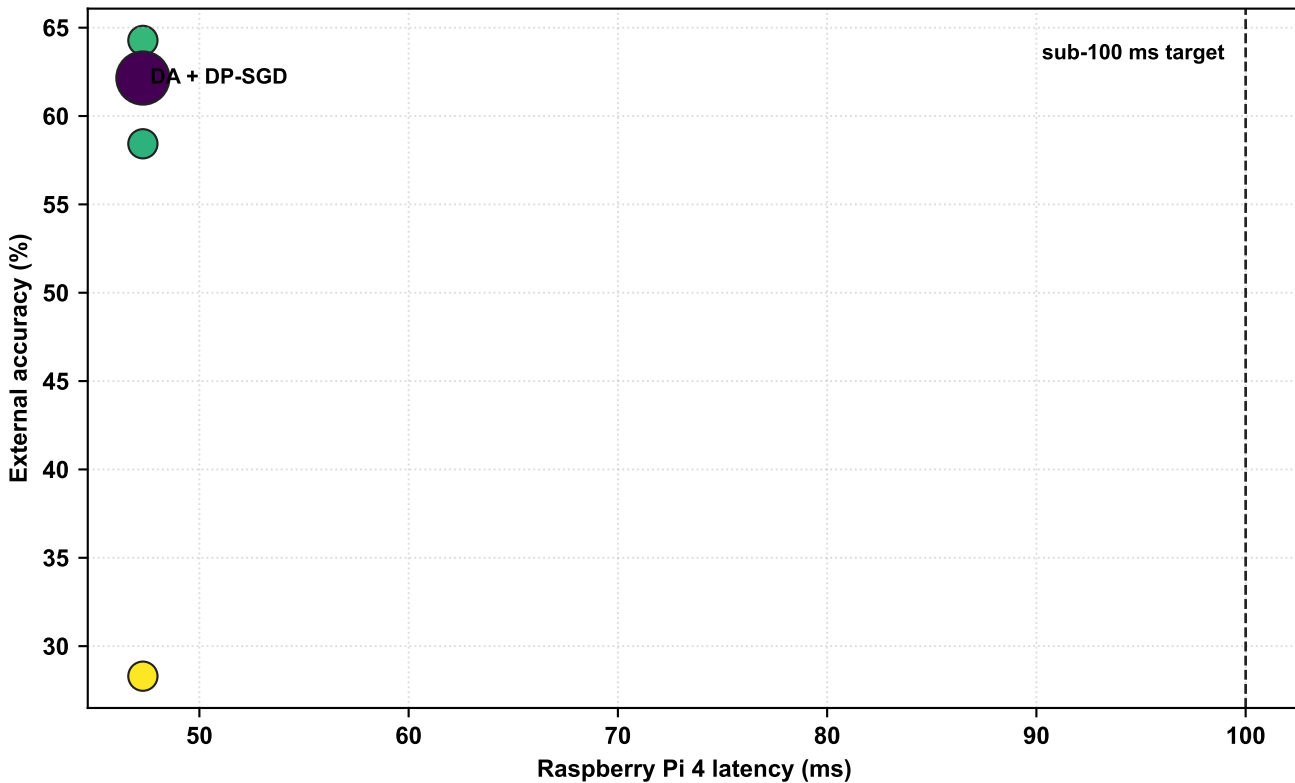
Figure 9. Privacy-Utility-Latency Trade-off
