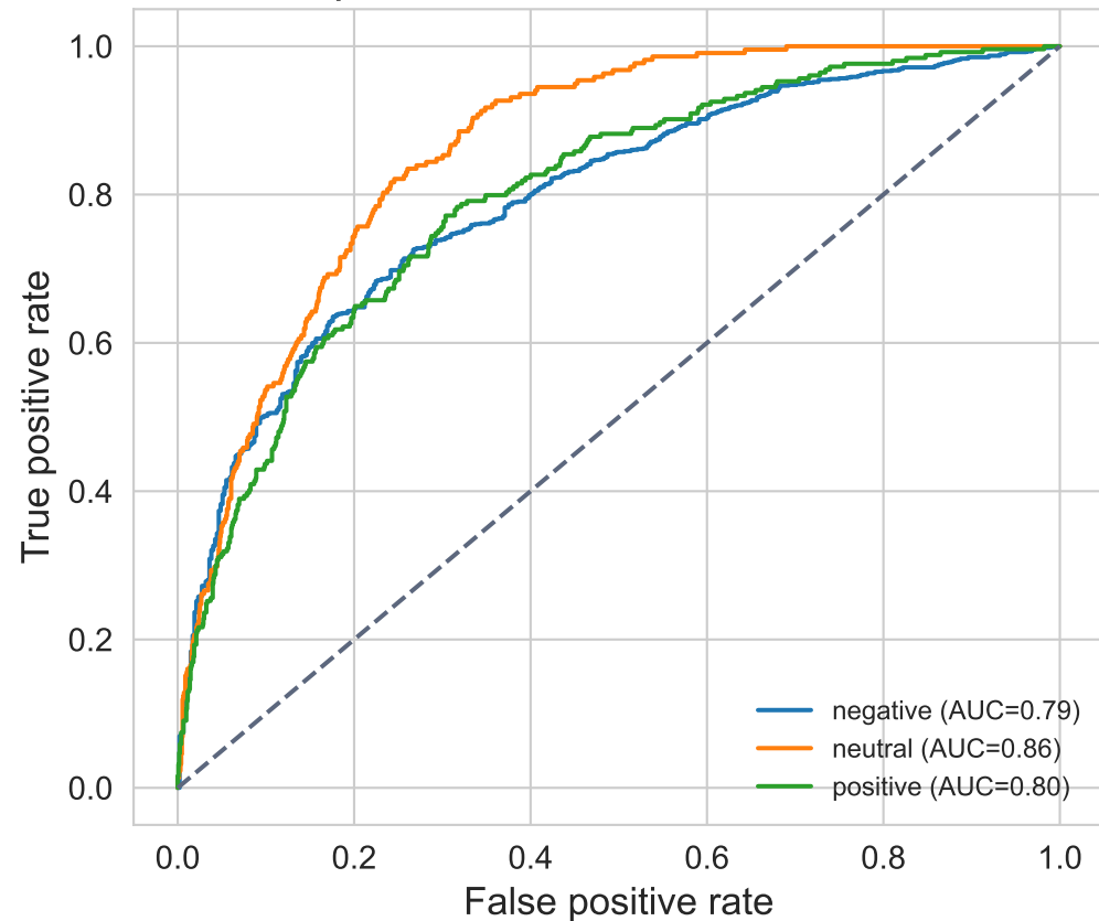
Speech Baseline ROC Curves
