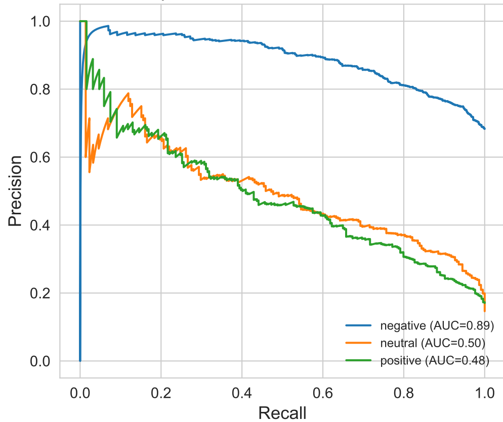
Speech Baseline PR Curves
