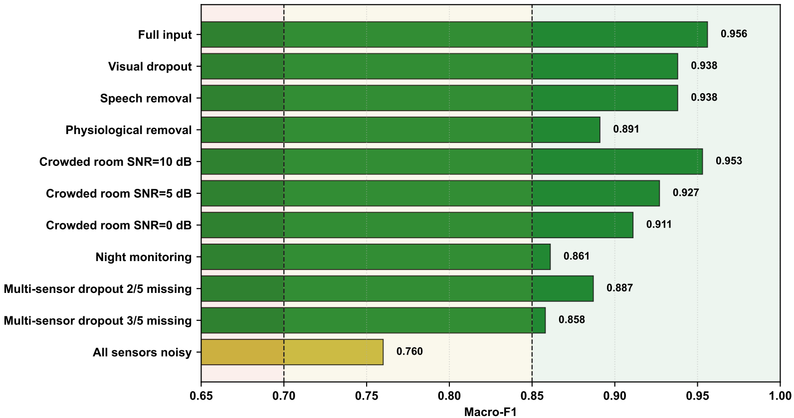
Figure 8. Missing-Modality Robustness
