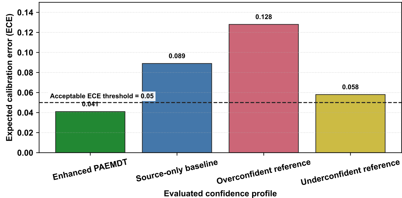
Figure 7. Expected Calibration Error Comparison
