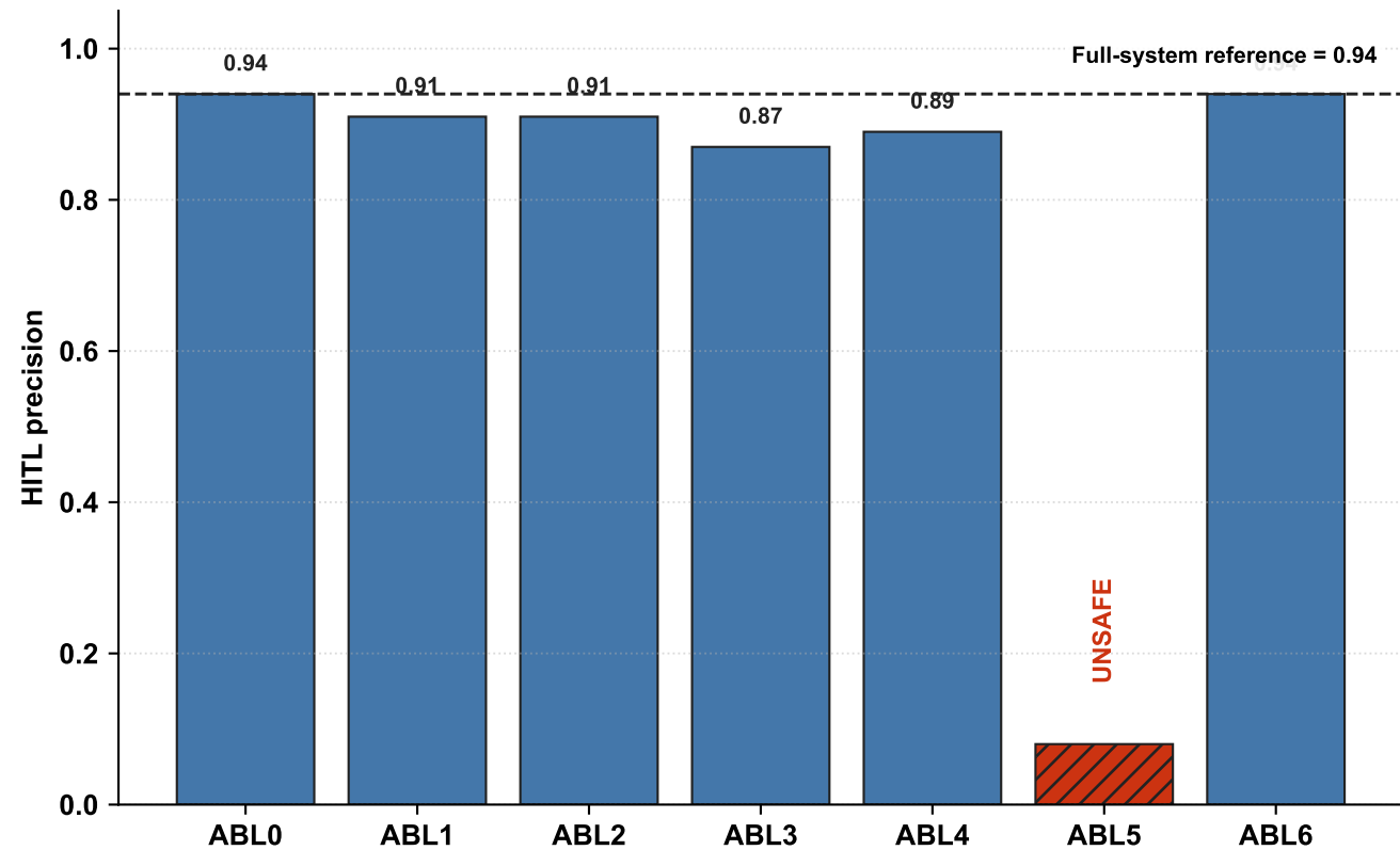
(b) HITL routing precision under component removal
