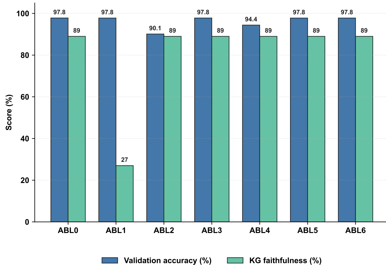
(a) Predictive performance and explanation faithfulness
