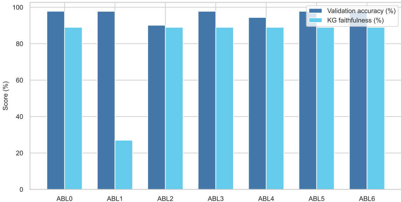
Figure 5A. Ablation study (predictive + explainability)
