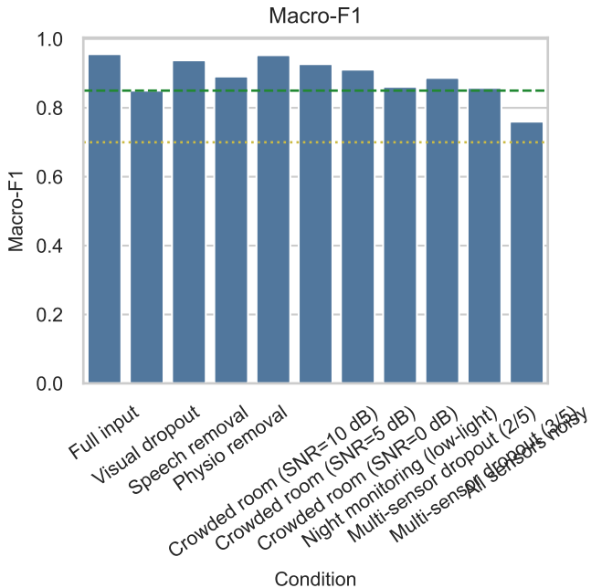
Figure 8. Missing-modality robustness
