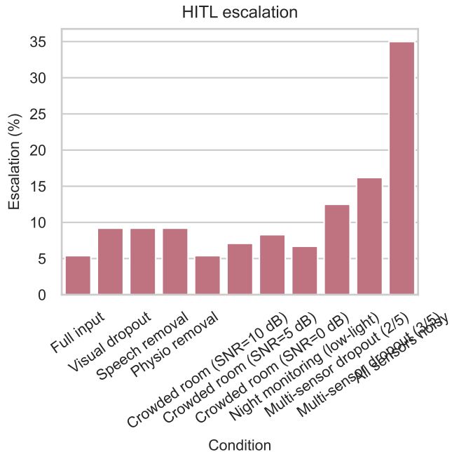
Figure 8. Missing-modality robustness
