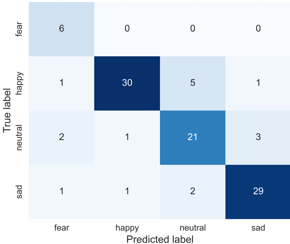
Vision Baseline Confusion Matrix
