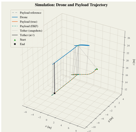
Figure 2: Simulation with EKF and payload control closed-loop: recovery from an initial perturbation, then trajectory tracking.
