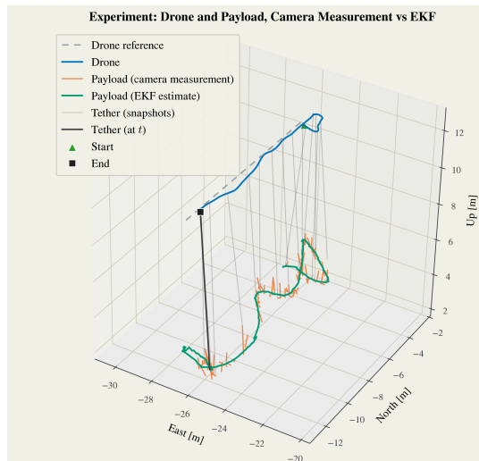
Figure 1: Drone tracking a trajectory with the payload as an unmodeled disturbance. EKF estimates are post-hoc; payload control is not yet closed-loop.
