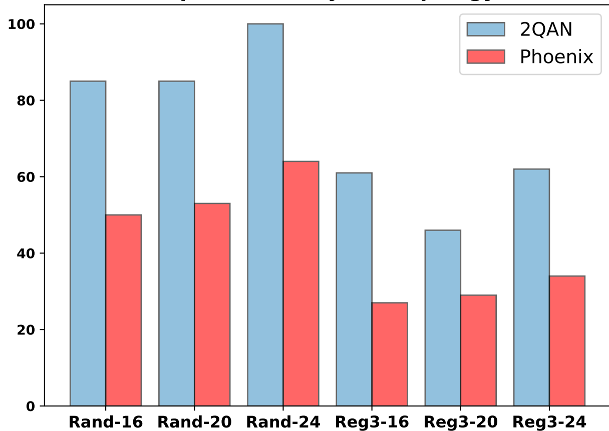
Depth-2Q (heavy-hex topology)
