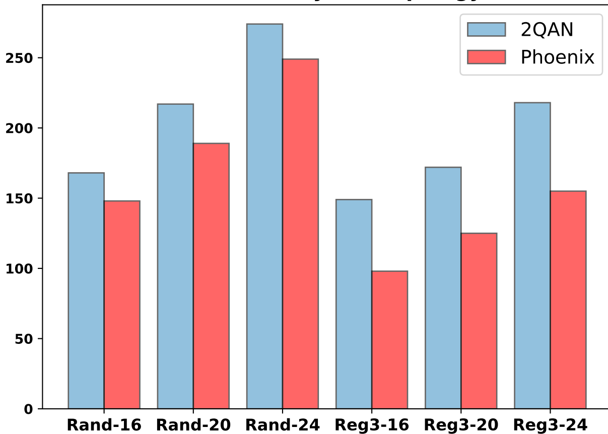
#CNOT (heavy-hex topology)
