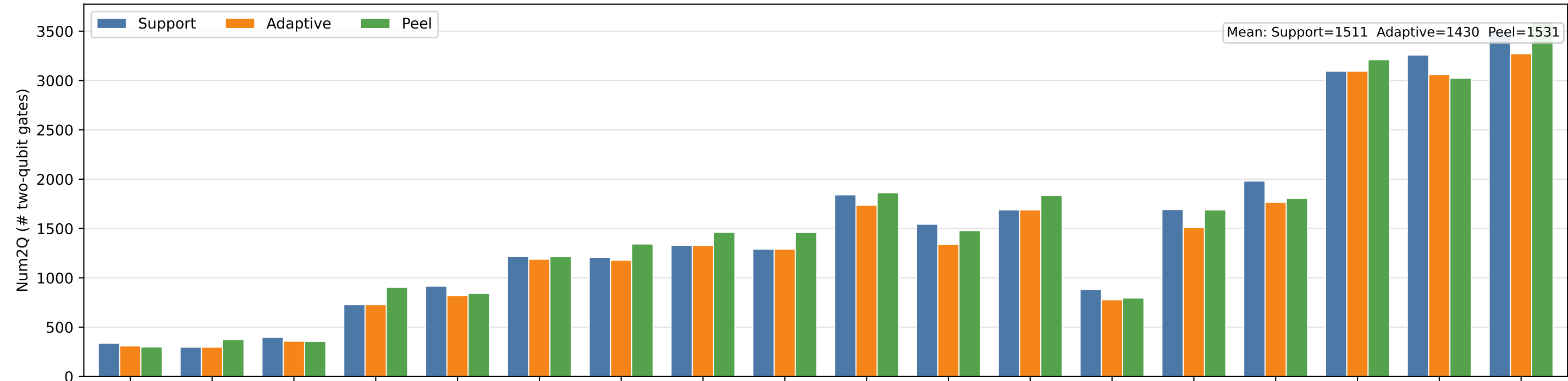
Support vs Adaptive vs Peel on UCCSD All-to-All Benchmarks
